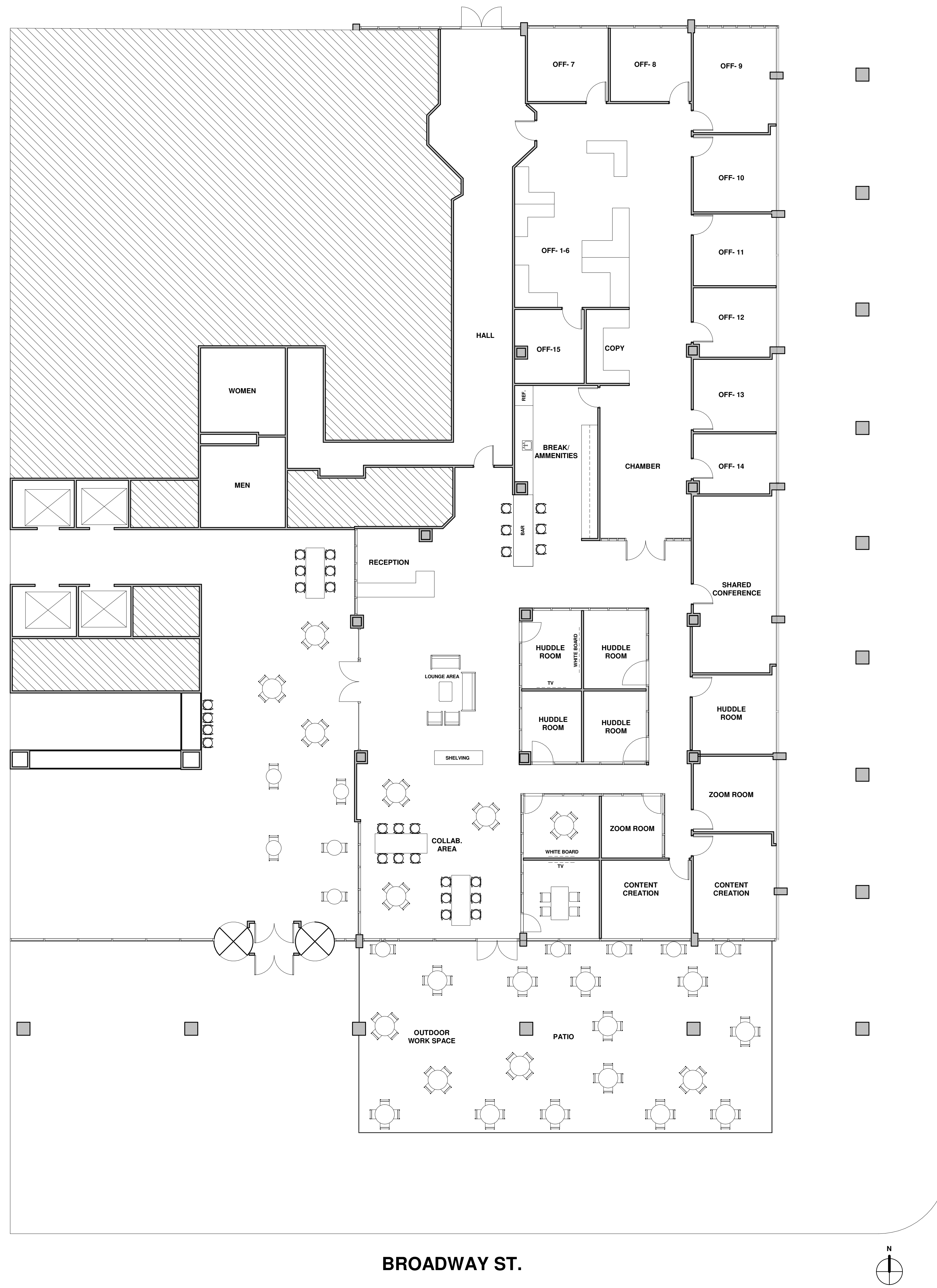
① Level 1 - FLOOR PLAN 1/8" = 1'-0"
